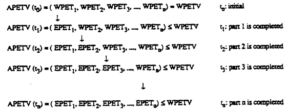
Figure 2: Transformation of the anticipated execution time vector.
