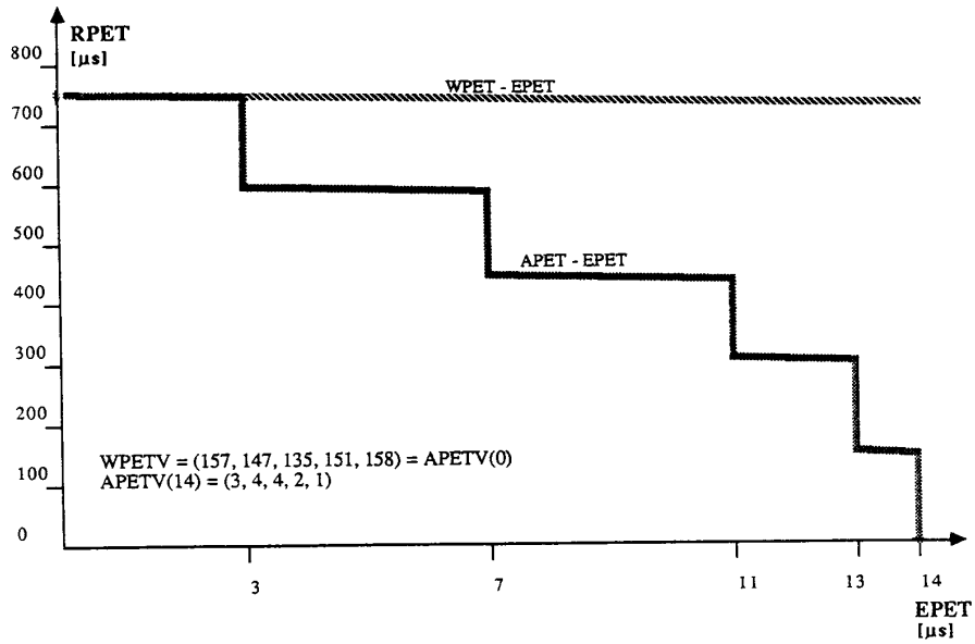
Figure 4: Computation of RPET based on WPET and APET: Example 1.
