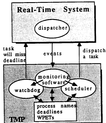
Figure 9: Software components residing in the TMP.
