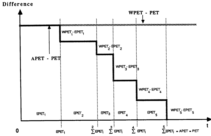
Figure 3: Differences between the cases of using WPET and APET.
