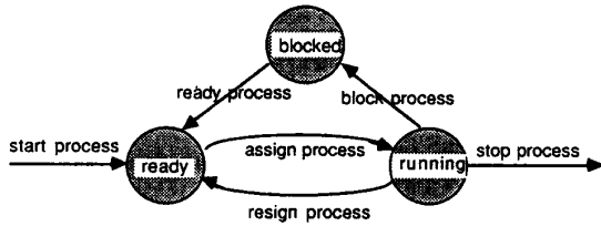
Figure 7: Events representing the operations of the dispatcher.
