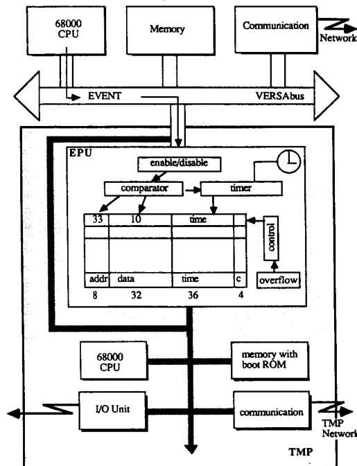
Figure 8: The TMP hardware.
