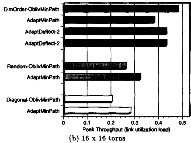
Figure 4: Peak throughput under bit-complement traffic
