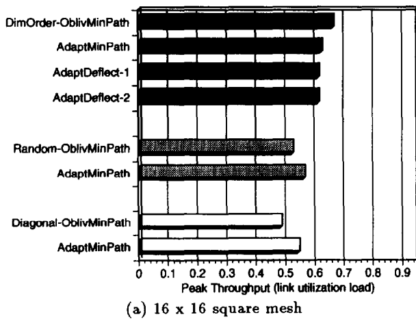
Figure 3: Peak throughput under node-uniform traffic
