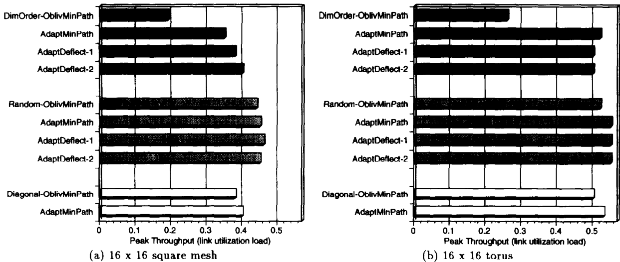
Figure 6: Peak throughput under matrix-transpose traffic
