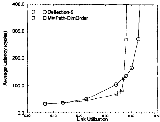
Figure 5: Minimal and nonminimal adaptive routing under bit-complement traffic
