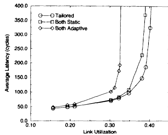
(b) Bit-complement traffic
