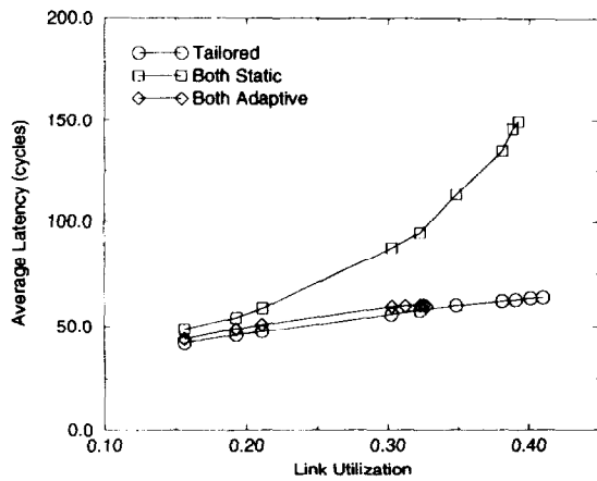
(a) Bit-reversal traffic
