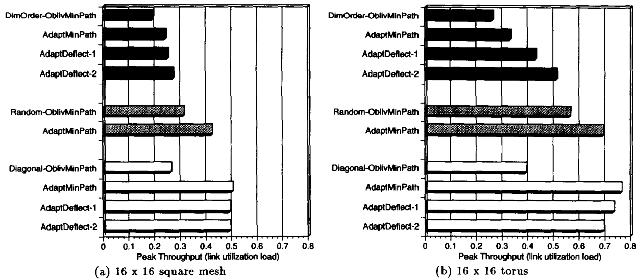
Figure 7: Peak throughput under bit-reversal traffic
