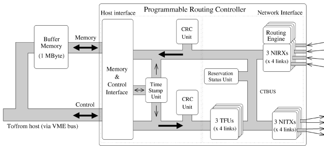
Fig. 3. PRC architecture.
