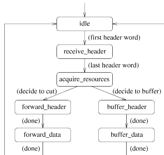
(a) Receiver state machine
