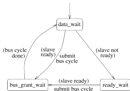
(b) Bus interface control
