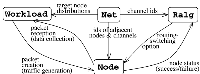
Fig. 1. Structure of pp-mess-sim .
