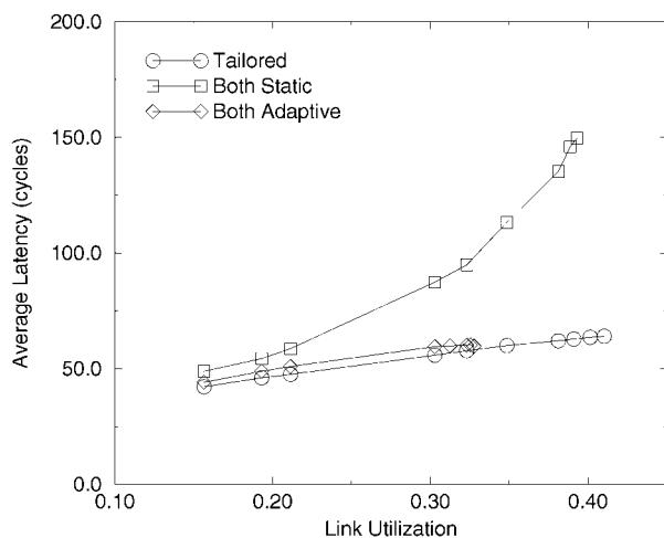
(a) Bit-reversal traffic
