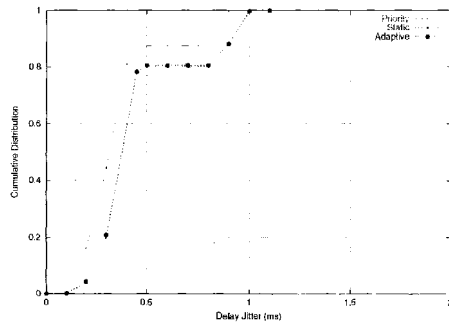
Fig. 7. Delay jitter in over-provisioning scenario
