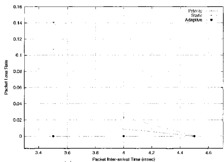
Fig. 3. Packet-loss rate
