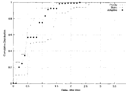
Fig. 5. Delay jitter in under-provisioning scenario
