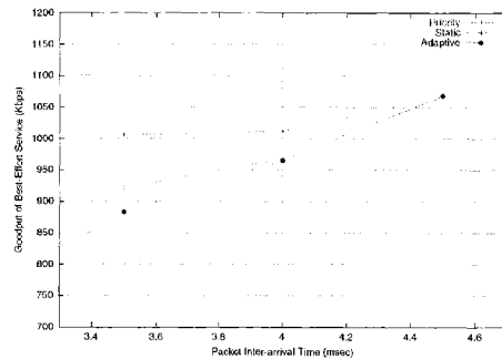
Fig. 9. Goodput of best-effort service
