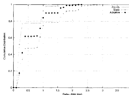
Fig. 6. Delay jitter in on-provisioning scenario
