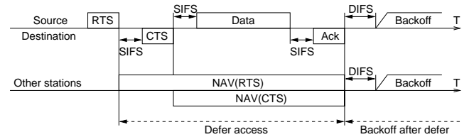
Figure 4: NAV setting during a four-way frame exchange
