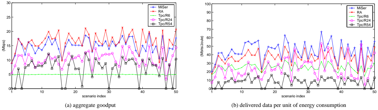
Figure 13: Comparison for static random-topology networks (50 different scenarios)
