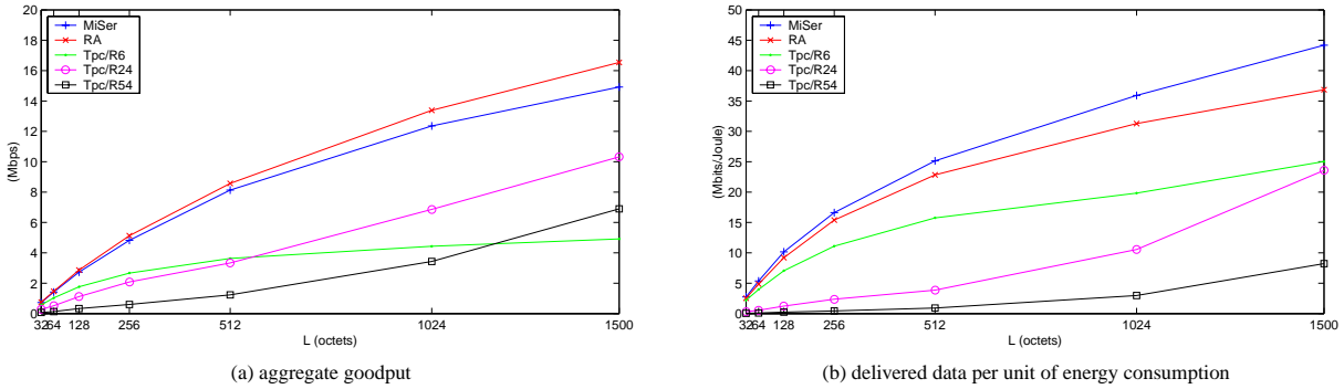
Figure 15: Comparison for various data payloads (average over 50 random topologies)
