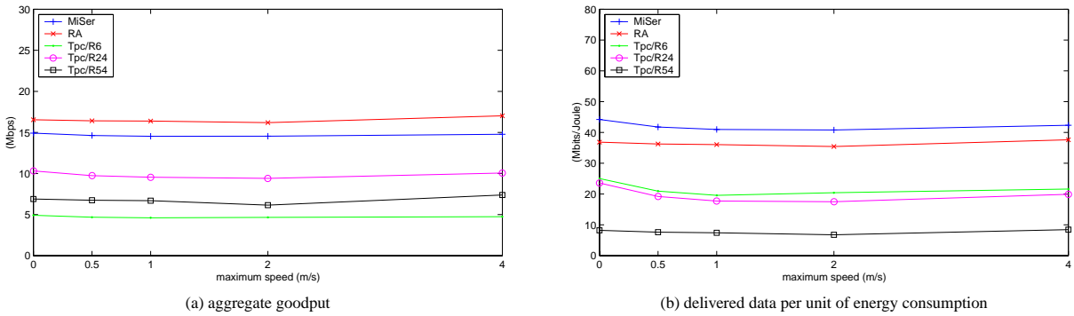
Figure 14: Comparison for various station mobility patterns (average over 50 random topologies)
