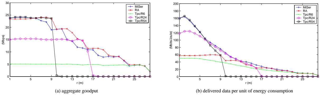
Figure 12: Comparison for static star-topology networks (various radius)
