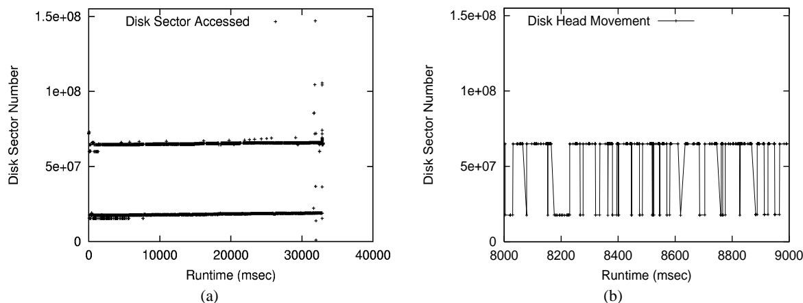
Figure 1: Part (a) shows disk sectors that were accessed when executing a cvs -q update command within a CVS local directory containing the Linux 2.6.7 source code. Part (b) shows the disk head movement within a 1-second window of the disk trace shown in part (a).
