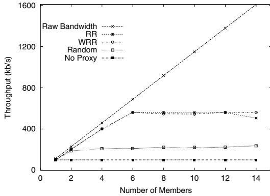
Fig. 2. Simulation result of TCP throughput.
