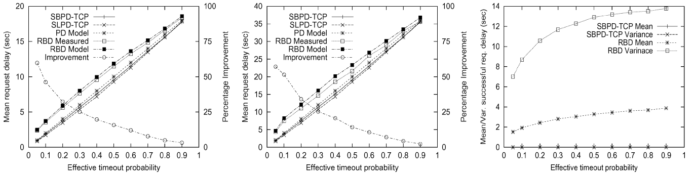
Fig. 6. Request delay comparison. (left) Delay for \lambda_0 = 60 clients/s and T_{\text{abort}} = 20 s. (center) Delay for \lambda_0 = 80 clients/s and T_{\text{abort}} = 40 s. (right) Mean and variance for the delay of successful requests (same configuration as left).
