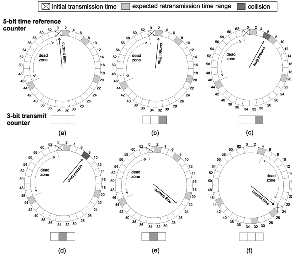
Fig. 5. Example of request classification based on the time reference and transmit counters. (a) Initial drop. (b) Retransmission drop. (c) Collision detected without time overlap. (d) Collision detected with time overlap. (e) Packet does not get retransmitted and drop counter remains the same. (f) Collision detected and new transmission overwrites old one.
