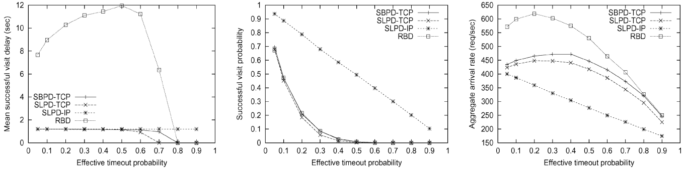
Fig. 7. User-visit behavior. In all cases, \lambda_0 = 60 clients/s and T_{\text{abort}} = 20 s. (left) Mean successful visit delay (a point with zero value implies that no visit was successful). (center) Probability of successful visit. (right) Effective arrival rate.
