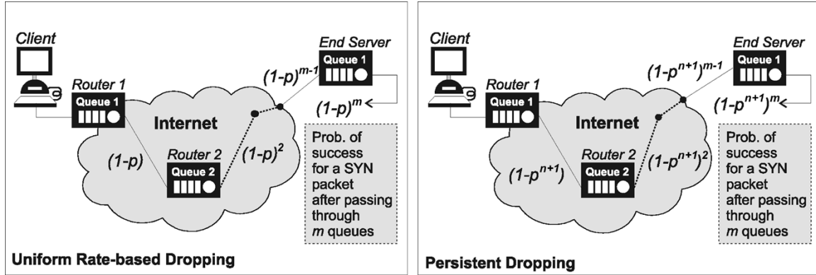
Fig. 3. Probability of success in network of queues.
