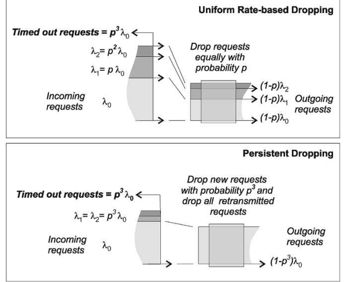
Fig. 2. Illustrative comparison between rate-based dropping and PD. We view the outgoing link as a smaller pipe than the stream of incoming requests. We then show how the two strategies drop incoming requests to fit them into the pipe.
