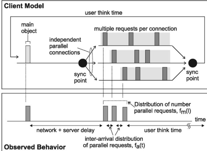
Fig. 1. Persistent client model.
