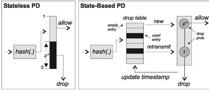
Fig. 4. Stateless and state-based implementation of persistent drop controller.
