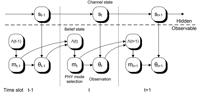
Fig. 5. A graphical model of the POMDP for PHY mode adaptation
