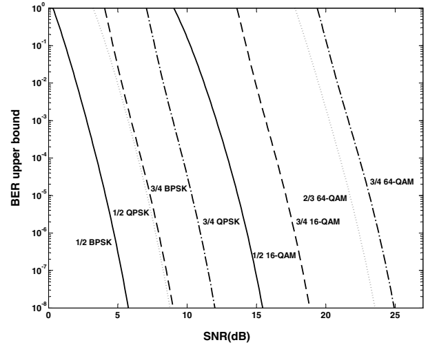
Fig. 4. BER upper bounds of the IEEE 802.11a PHY modes
