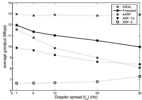
Fig. 8. Comparison of goodput among various rate adaptation schemes
