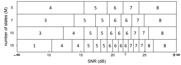
Fig. 12. The optimal PHY control policies for MDP with various numbers of FSMC states under the good channel condition
