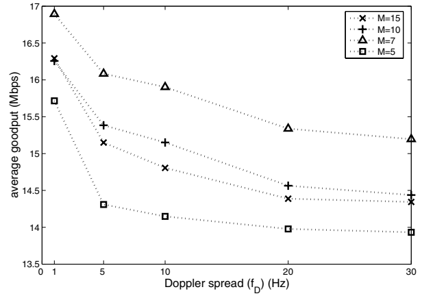
Fig. 11. Achieved goodput of the proposed scheme with various numbers of states under the good channel condition
