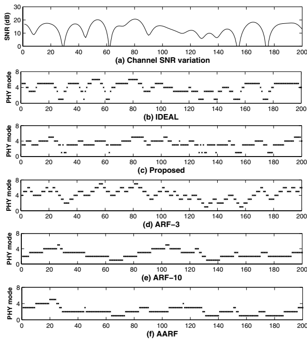
Fig. 13. Comparison of PHY mode adaptation of the schemes under consideration
