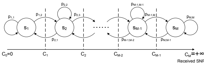
Fig. 1. Finite-state Markov channel (FSMC) model for a Rayleigh fading channel in IEEE 802.11 WLANs
