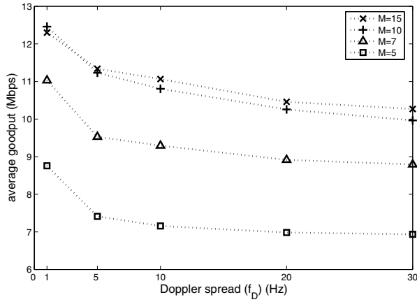
Fig. 9. Achieved goodput of the proposed scheme with various numbers of FSMC states under the normal channel condition
