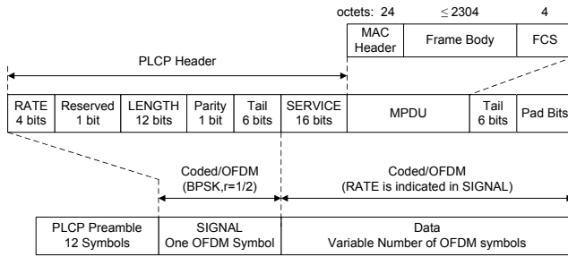
Fig. 2. PPDU frame format of the IEEE 802.11a PHY
