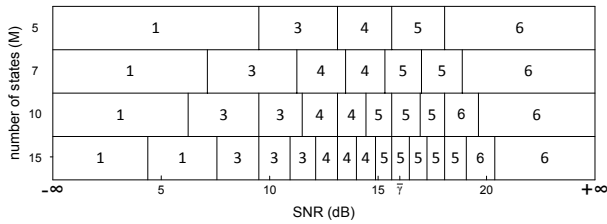
Fig. 10. The optimal PHY control policies for MDP with various numbers of FSMC states under the normal channel condition
