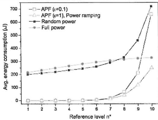
Figure 4. Comparison of energy consumption for initial access ( G = 0.75 ).
