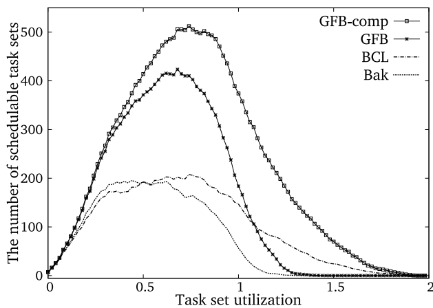
(a) m = 2 , tests with low time-complexity
