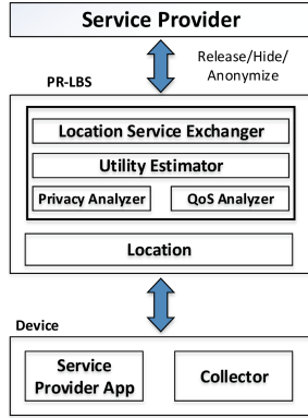
Fig. 3. The high-level operations of PR-LBS.
