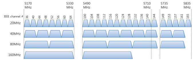
Fig. 1. Channelization of 802.11ac in the USA.
