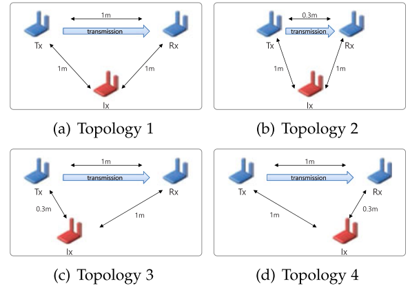
Fig. 7. Experimental topologies.
