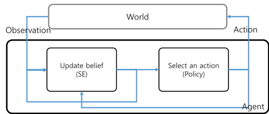
Fig. 11. A POMDP model. The POMDP agent can be decomposed into a state estimator (SE) and a policy.
