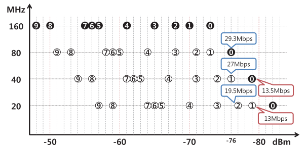
Fig. 4. Ideal MCS levels on each bandwidth according to receiver sensitivity, where the number inside each circle indicates the corresponding MCS level and the x -axis represents the required receiver sensitivity in decreasing order.
