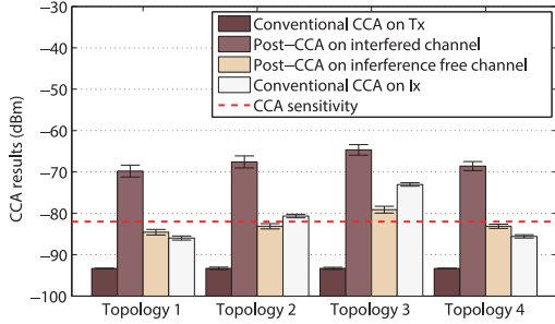
(a) Conventional CCA and Post-CCA results on both of half bandwidth channels at Tx, and CCA results at Ix while Tx is transmitting
