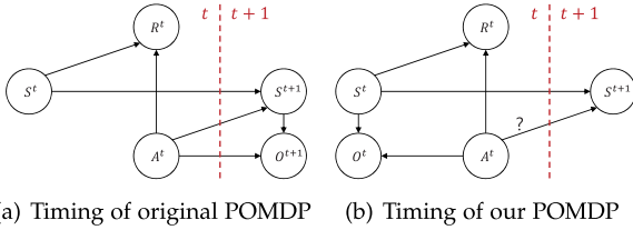
Fig. 13. A modification on the timing of POMDP to fit our problem.
