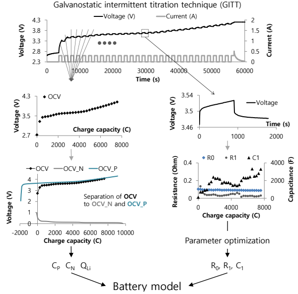
Figure 7: Model-based battery diagnosis
