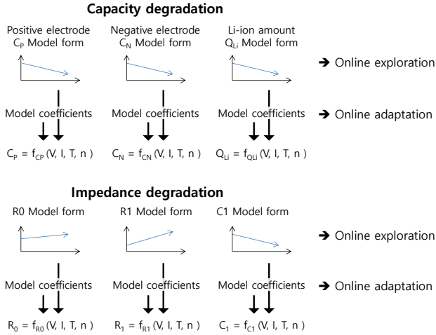
Figure 6: Proposed modeling of battery degradation.
