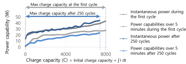
Figure 14: Example total capacity and power capability degradations. After 250 cycles, the battery’s energy capacity and power capability over 5 minutes decrease.
