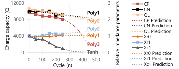
Figure 10: Example model parameter degradations during 250 discharge/charge cycles. Operating temperature is 23^\circ C , battery C-rate is 2,300mA, charge current is 2A, max voltage is 4.2V, average discharge current ( E(I_d) ) is 2A, and the root mean square of discharge current ( RMS(I_d) ) is 2.45A. Dotted lines show the degradation predictions of model parameters. These graphs are obtained with evaluation process to be described in Section VI.
