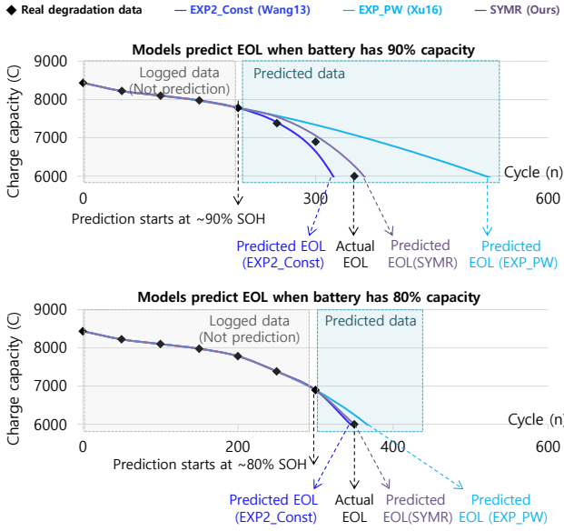
Figure 18: Examples of EOL prediction at different SOH
