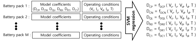
Figure 13: Development of the parameter degradation rate function based on parameter degradation and operating condition profiles.
