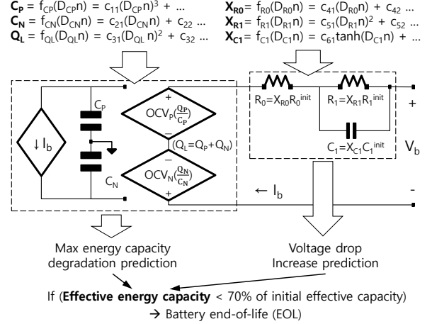
Figure 15: Battery EOL prediction based on the battery model and the model parameter degradation function
