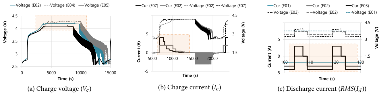
Figure 21: Test profiles with different charge/discharge currents and voltages.
