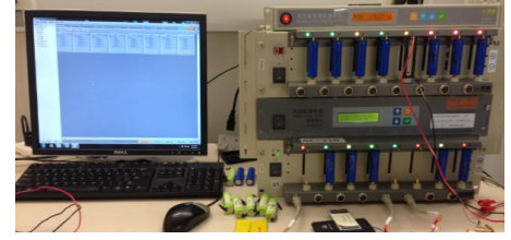
Figure 17: Neware battery tester
