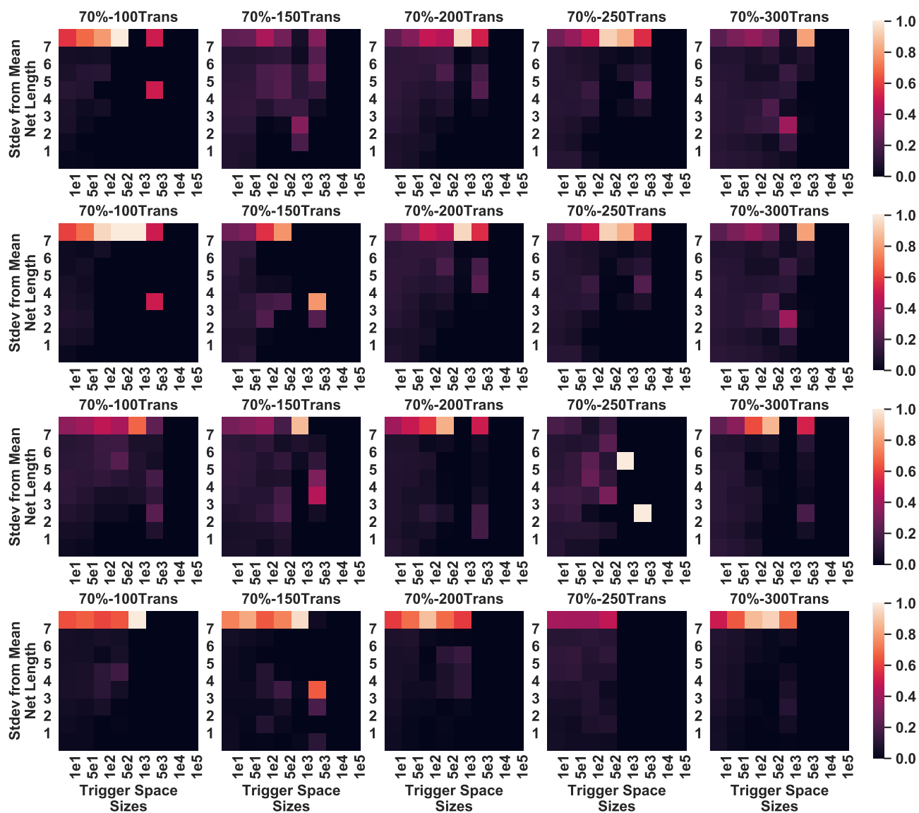
Fig. 14. Route Distance Metric for ORI200 at 70% Density. Same as Fig. 13, except a target density of 70% was held across each layout.
