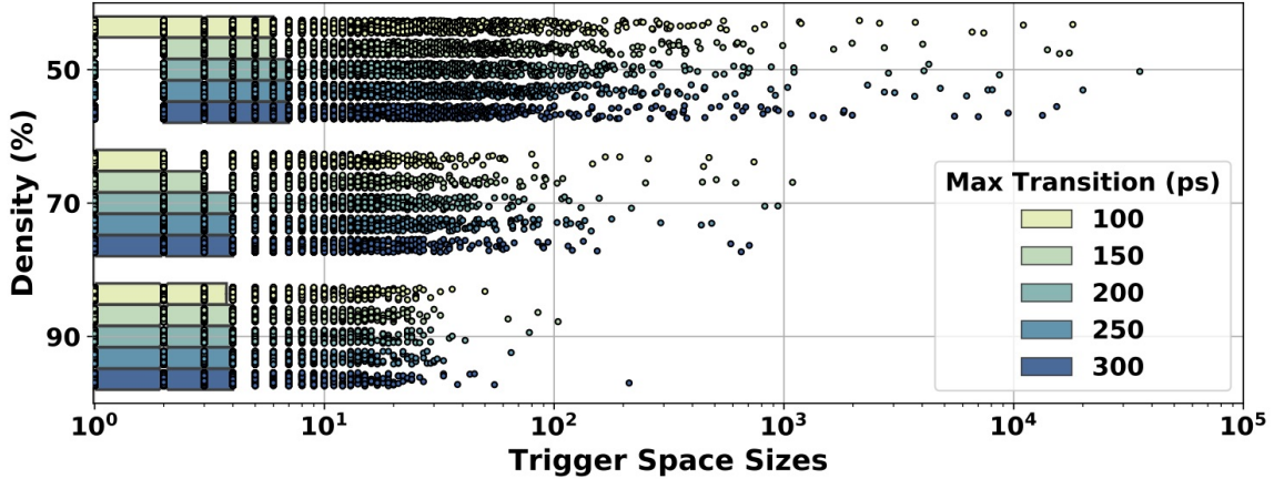
Fig. 8. Trigger Space distributions for 15 different OR1200 processor IC layouts. Core density and max transition time parameters are varied across the layouts, while target clock frequency is held constant at 1 GHz. The boxes represent the middle 50% (interquartile range or IQR) of open placement regions in a given layout, while the dots represent individual open placement region sizes.
