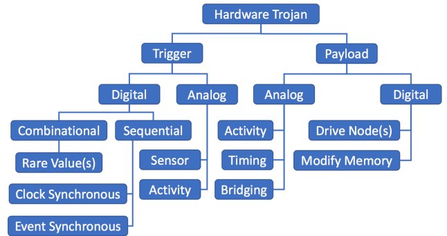
Fig. 3. An existing taxonomy of hardware Trojans [26]. This taxonomy classifies hardware Trojans based on their trigger and payload types.
