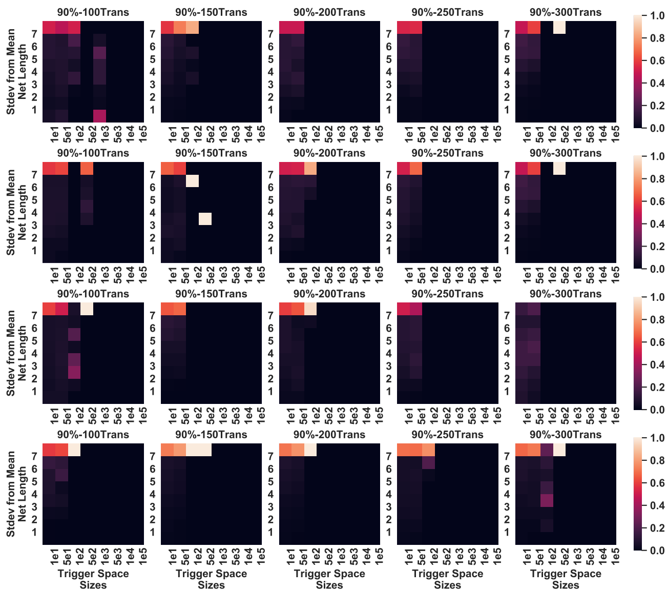
Fig. 15. Route Distance Metric for ORI200 at 90% Density. Same as Fig. 13, except a target density of 90% was held across each layout.
