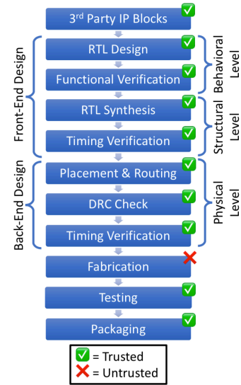
Fig. 1. The typical IC design process starts with a textual specification of design requirements and ends with a fabricated and tested chip. Green check-boxes mark trusted stages and red x-boxes mark the untrusted step (i.e., an untrusted foundry). The fabrication step takes a GDSII file (physical IC layout) as input and produces a wafer of die. While prior work proposes metrics for untrusted front-end design [17], [21]–[23], no mechanism exists for measuring an IC layout’s resilience to an untrusted foundry.
